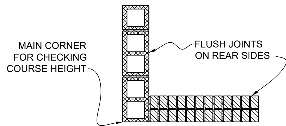
G COURSE 11 3/4"=1'-0"
