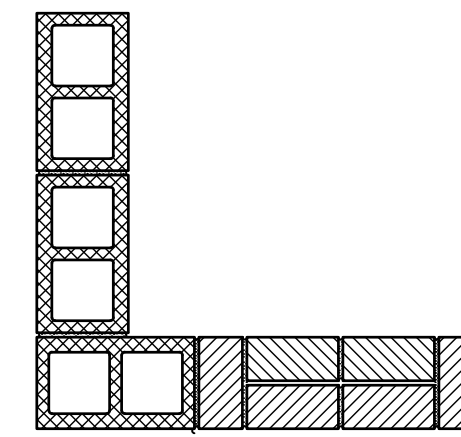
J COURSE 2,8,14 3/4"=1'-0"
