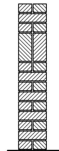
E SECTION 3/4"=1'-0"
