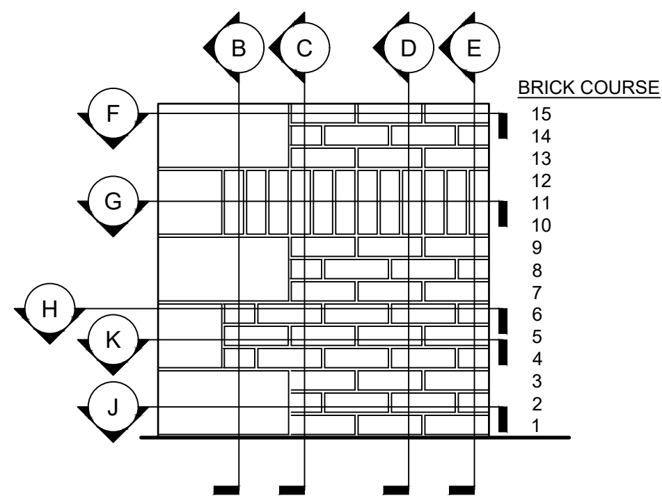
RIGHT VIEW 3/4"=1'-0"
