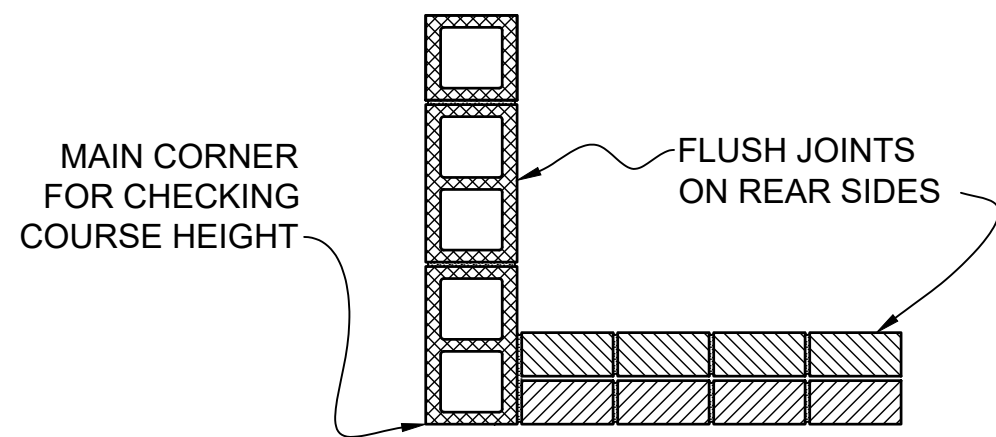
K COURSE 5 3/4"=1'-0"
