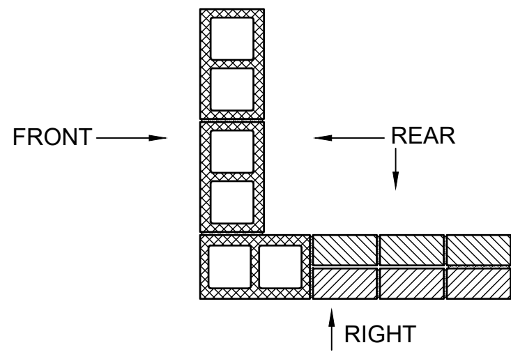
F COURSE 1,3,7,9,13,15 3/4"=1'-0"
