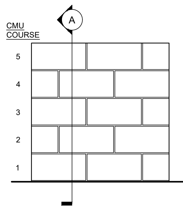
FRONT VIEW 3/4"=1'-0"
