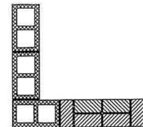
J COURSE 2,8,14 3/4"=1'-0"
