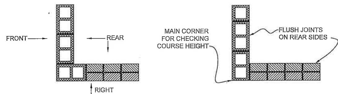
F COURSE 1,3,7,9,13,15 3/4"=1'-0"
