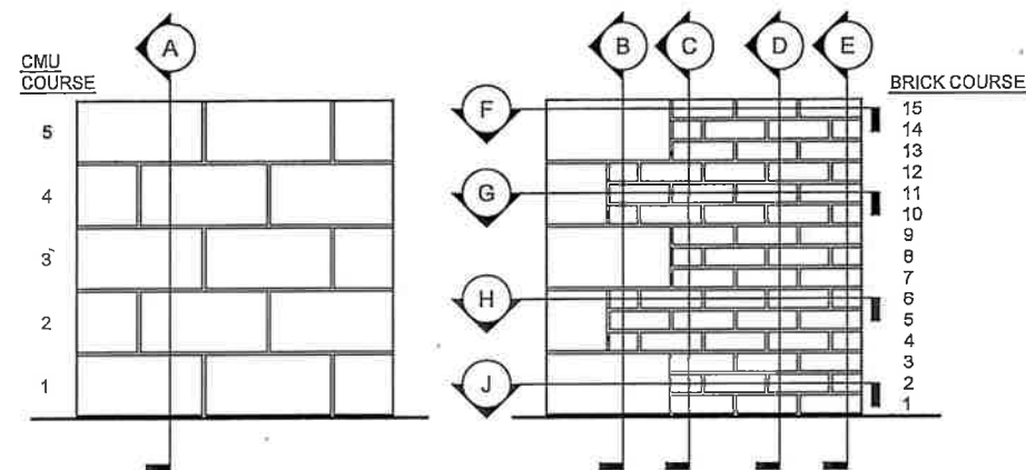
FRONT VIEW 3/4"=1'-0"
